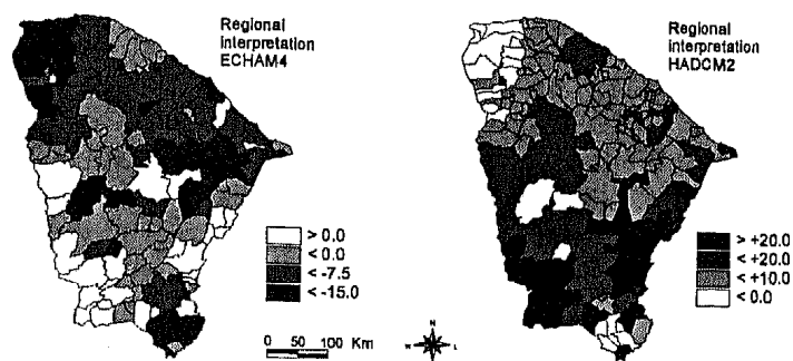
Figure 5. Regional interpretations of GCM results for precipitation trends (%) in Ceará over the period 2001 to 2050, assuming continued growth of atmospheric greenhouse gas concentrations
