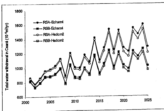
Figure 9. Total water withdrawals in Ceará between 2001 and 2025: as computed by the regional water use model NoWUM for the two reference scenarios RS A and RS B, using climate scenarios based on the climate models ECHAM4 and HadCM2
