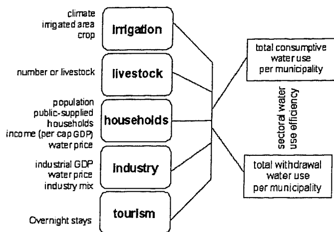
Figure 3. Overview of the regional-scale water use model NoWUM; on the left-hand side, the driving forces of water use in the five sectors are indicated
