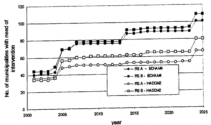
Figure 11. Number of municipalities with need of intervention due to water stress in Ceará for four scenarios in the period 2001 to 2025
