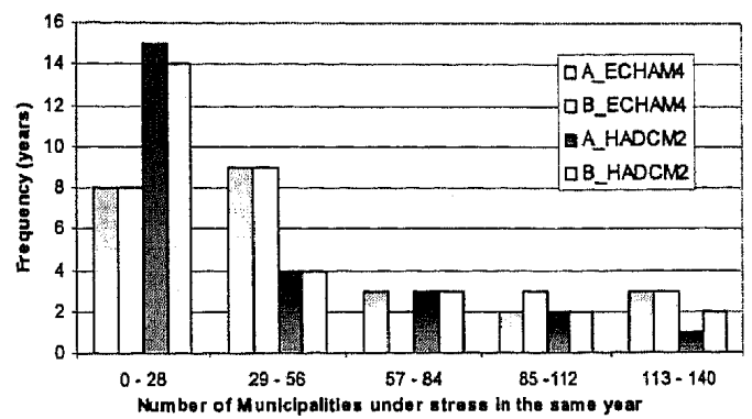
Figure 10. Histogram of municipalities under water stress in Ceará (2001 to 2025) for four scenarios
