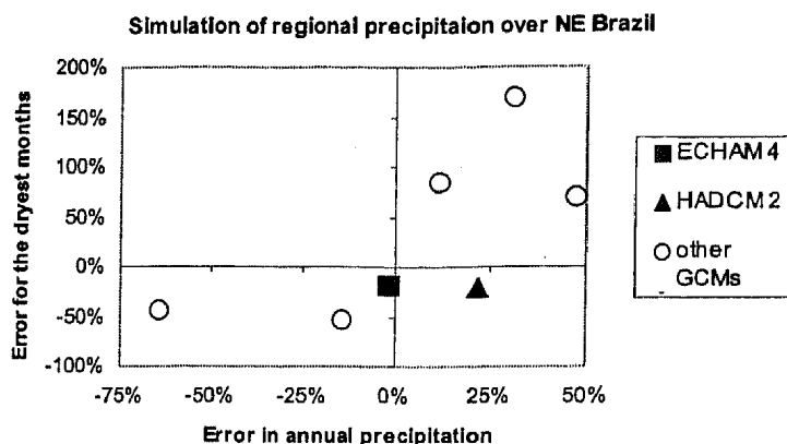
Figure 4. Simulation of regional precipitation over semiarid Northeast Brazil in the period 1961 to 1990 by seven GCMs compared to the observational database (New et al., 1999)
