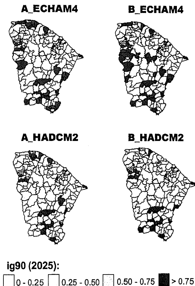
Figure 13. Water stress ( ig_{90} ) in all municipalities in Ceará for year 2025 for four scenarios
