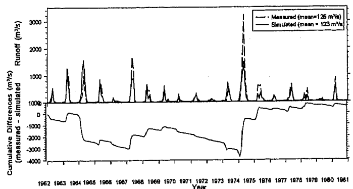
Figure 8. Runoff at station Peixe Gordo (Jaguaribe River, Ceará, Brazil); catchment area: 47,500 km 2 ; monthly values, measured and simulated with WASA
