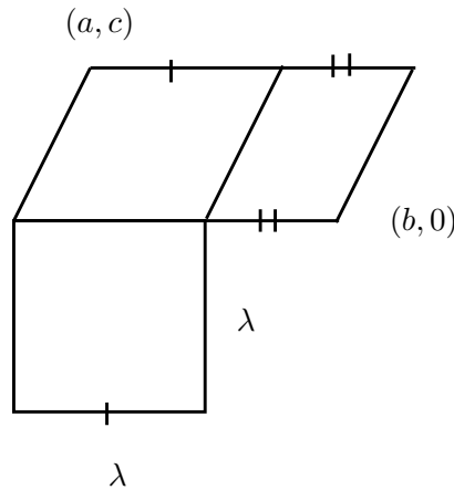
FIGURE 1. A translation surface attached to a splitting prototype
