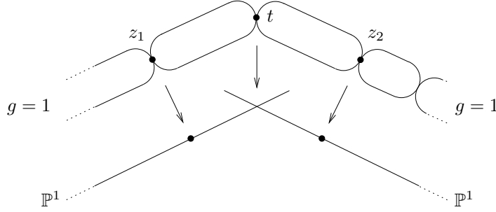
FIGURE 2. Admissible double cover for a reducible degeneration with z_i a Weierstrass point
