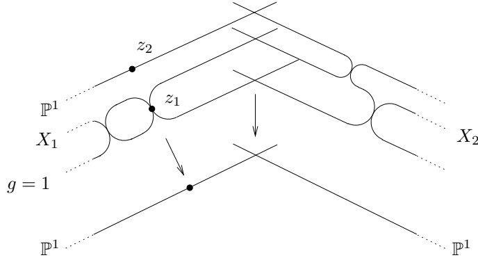
FIGURE 3. Admissible double cover for a reducible degeneration of type (g_1, g_2, n) = (1, 1, 2)
