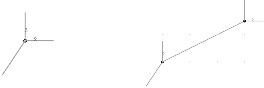
FIGURE 1. Tropicalization of an elliptic curve in Weierstraß form. The left hand side shows the case 3v(a) \geq 2v(b) , the right hand side the case 3v(a) < 2v(b) . The numbers on the edges indicate the tropical multiplicities. If no number is given, the multiplicity is one.
